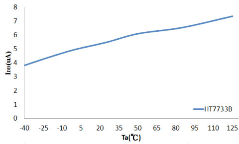
HT7733B I_{DD} vs. T_a
