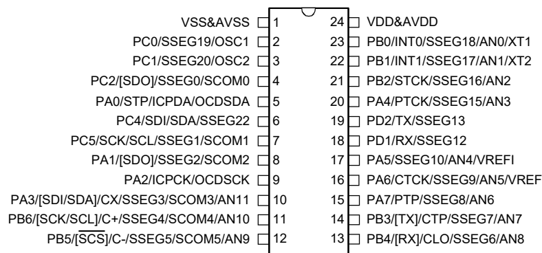
HT66F0195/HT66V0195 24 SOP/SSOP-A
