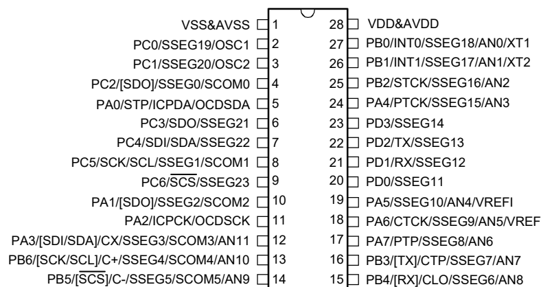
HT66F0195/HT66V0195 28 SOP/SSOP-A
