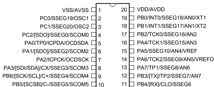
HT66F0186/HT66V0186 20 NSOP-A
