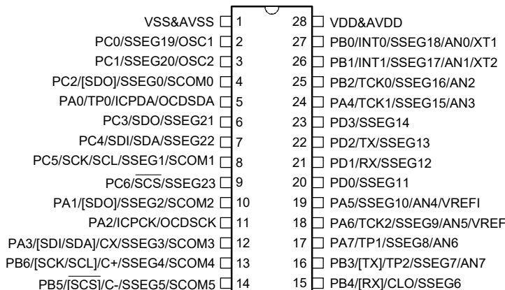
HT66F0186/HT66V0186 28 SOP-A/SSOP-A
