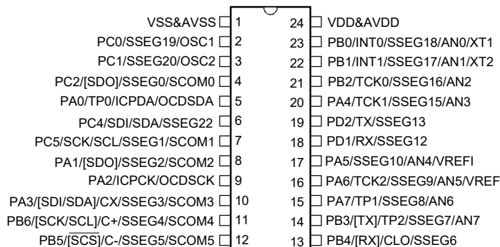
HT66F0186/HT66V0186 24 SOP-A/SSOP-A
