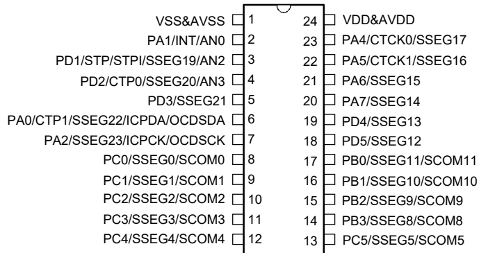
HT66F0184/HT66V0184 24 SOP-A/SSOP-A
