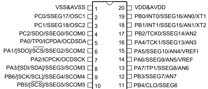
HT66F0175/HT66V0175 20 SOP-A/SSOP-A
