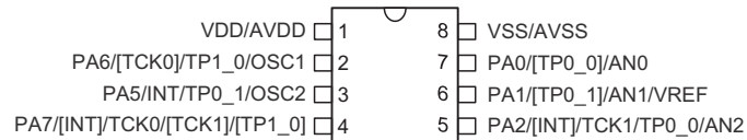
HT66F005/HT66F006 8 DIP/SOP-A
