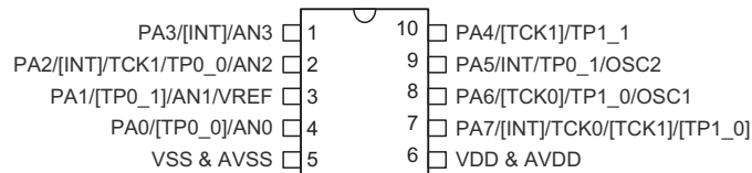
HT66F005/HT66F006 10 MSOP-A
