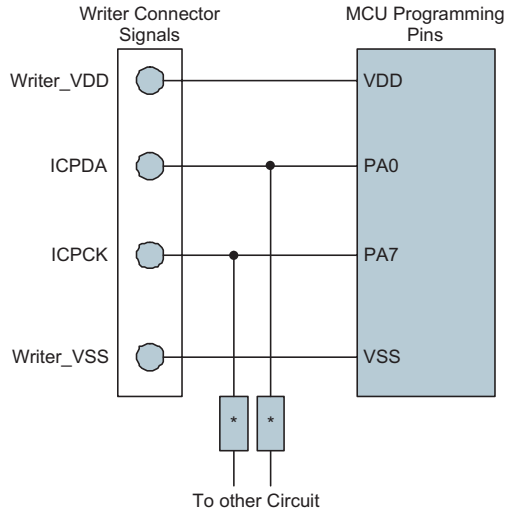
HT66F002/HT66F0025
