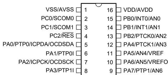
HT66F004/HT66V004 16 NSOP-A
