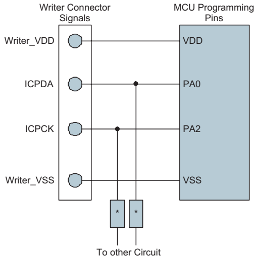
HT66F003/HT66F004
