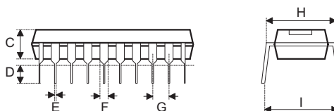
Fig2. 1/2 Lead Packages
