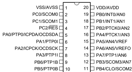
HT66F004/HT66V004 20 DIP-A/NSOP-A/SOP-A/SSOP-A
