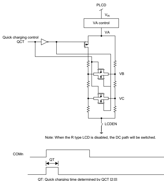
R 型偏压配置 – 1/3 Bias
