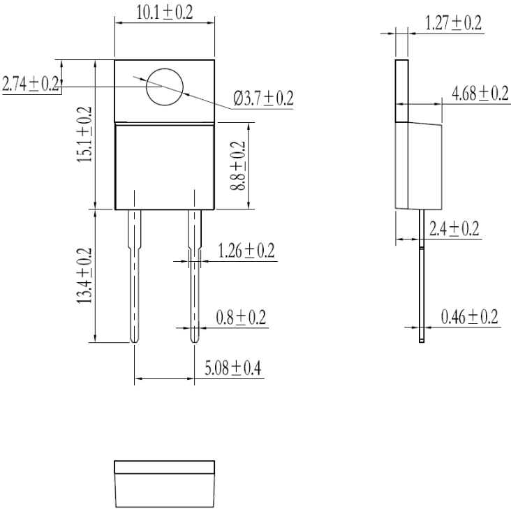
Dimensions in Millimeters Fig8. Package Outline
