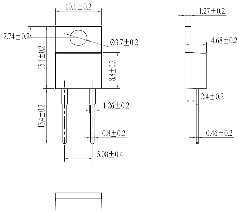
Dimensions in Millimeters Figure 8. Package Outline
