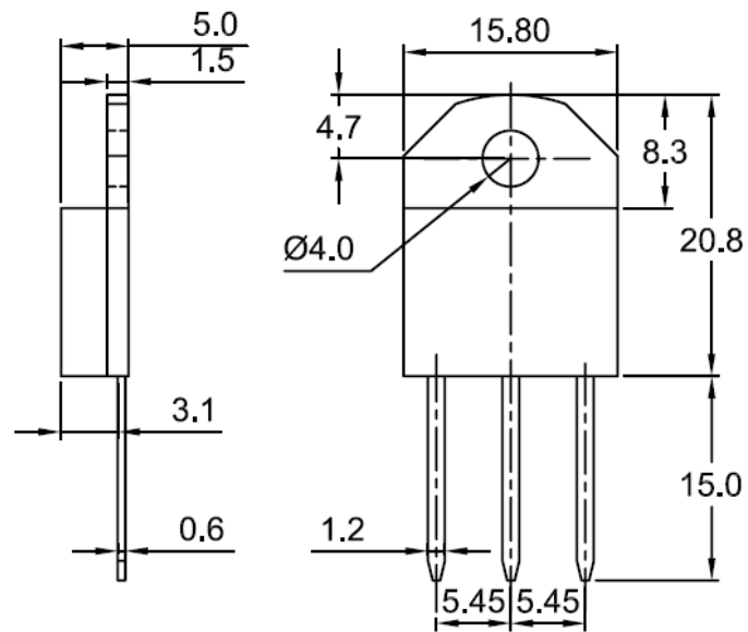
Dimensions in Millimeters Fig8. Package Outline
