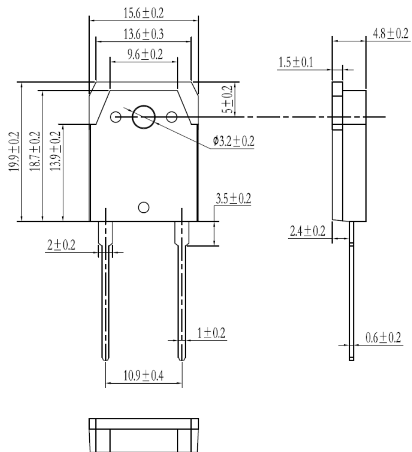
Dimensions in Millimeters Fig8. Package Outline
