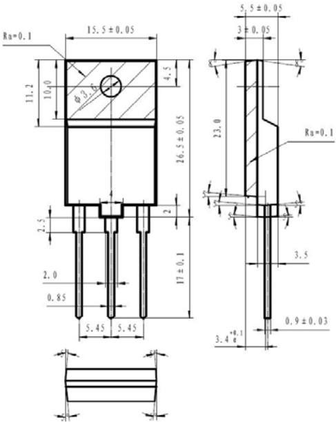
Figure7 Package Outline
