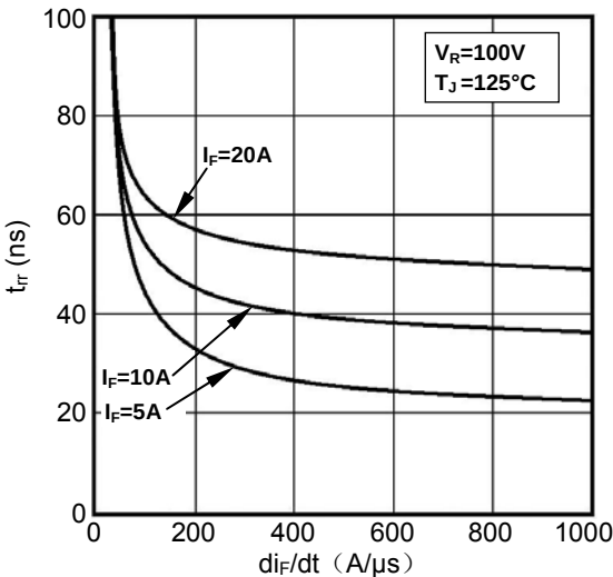
Fig2. Reverse Recovery Time vs di_F/dt
