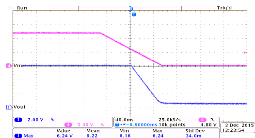
掉电响应: HT7560-7 ( I_{OUT}=150mA , T_{FALL}=100ms )
