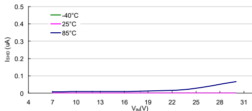
I_{SHD} vs V_{IN} : HT7560-7 ( I_{OUT}=0mA )
