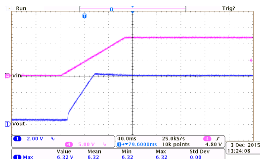
上电响应: HT7560-7 ( I_{OUT}=150mA , T_{RISE}=100ms )
