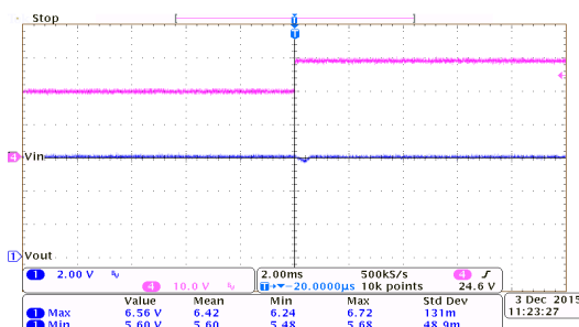
线性瞬态响应: HT7560-7 ( I_{OUT}=10mA )
