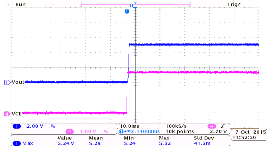
开关响应: HT7550-7 ( I_{OUT}=150mA , V_{CE}=0V to 2.7V)
