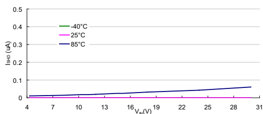
I_{SHD} vs V_{IN} : HT7533-7 ( I_{OUT}=0mA )
