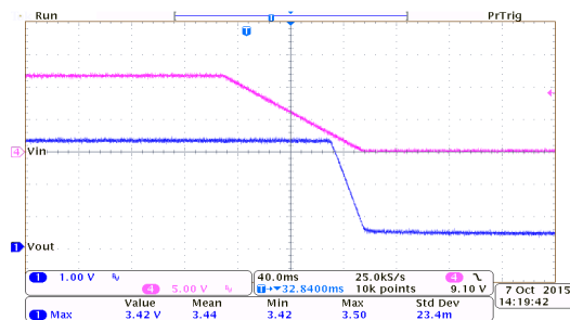
掉电响应: HT7533-7 ( I_{OUT}=0mA , T_{FALL}=100ms )
