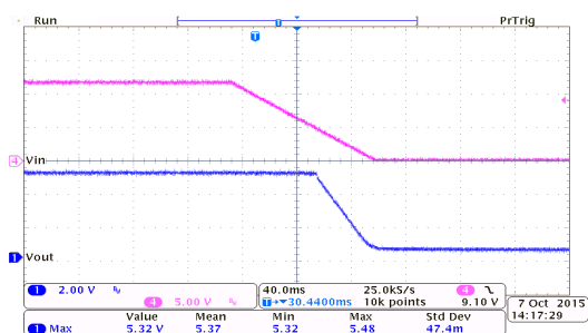
掉电响应: HT7550-7 ( I_{OUT}=150mA , T_{FALL}=100ms )
