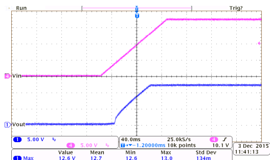
上电响应: HT75C0-7 ( I_{OUT}=150mA , T_{RISE}=100ms )
