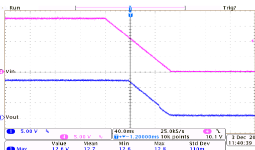
掉电响应: HT75C0-7 ( I_{OUT}=0mA , T_{FALL}=100ms )
