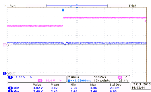
线性瞬态响应: HT7533-7 ( I_{OUT}=10mA )
