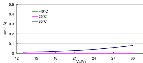
I_{SHD} vs V_{IN} : HT75C0-7 ( I_{OUT}=0mA )
