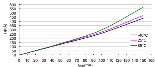
I_{SS} vs I_{OUT} : HT7560-7 ( V_{IN}=8.0V )
