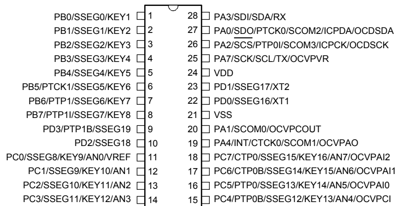
BS87C16A-3/BS87CV16A 28 SOP-A
