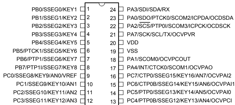
BS87C16A-3/BS87CV16A 24 SOP-A
